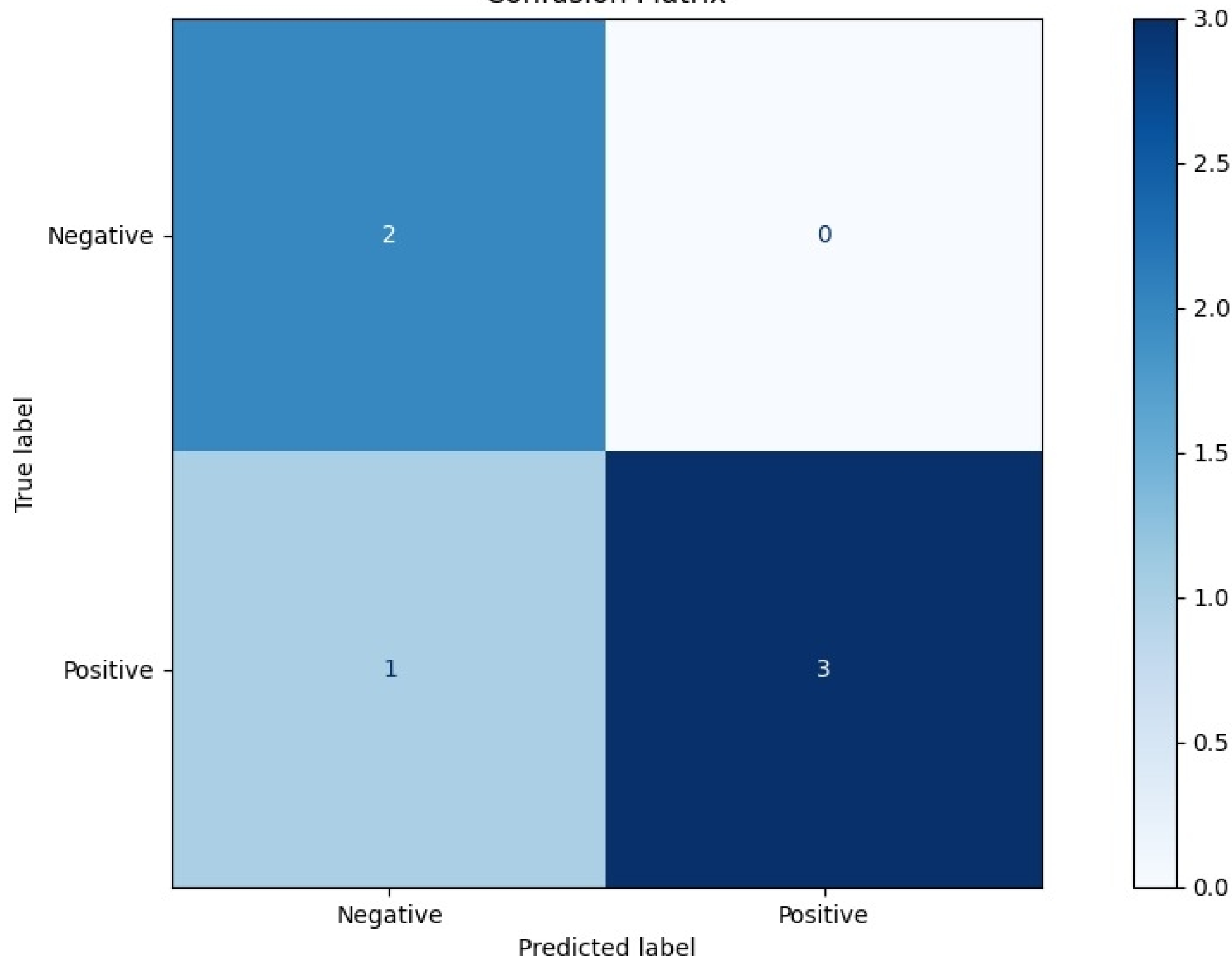
Confusion Matrix
